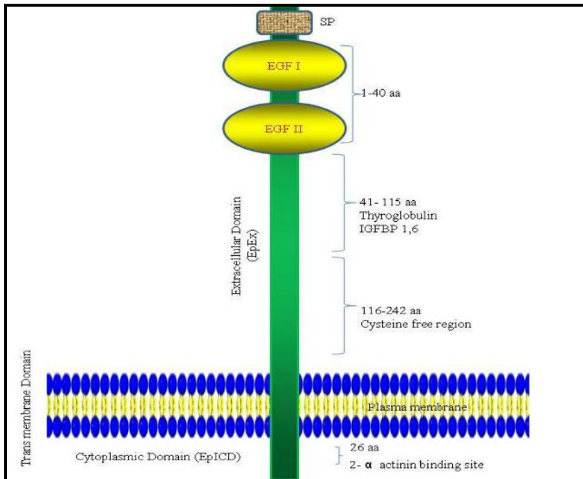
Figure (1): Schematic diagram of EpCAM structure [3].
