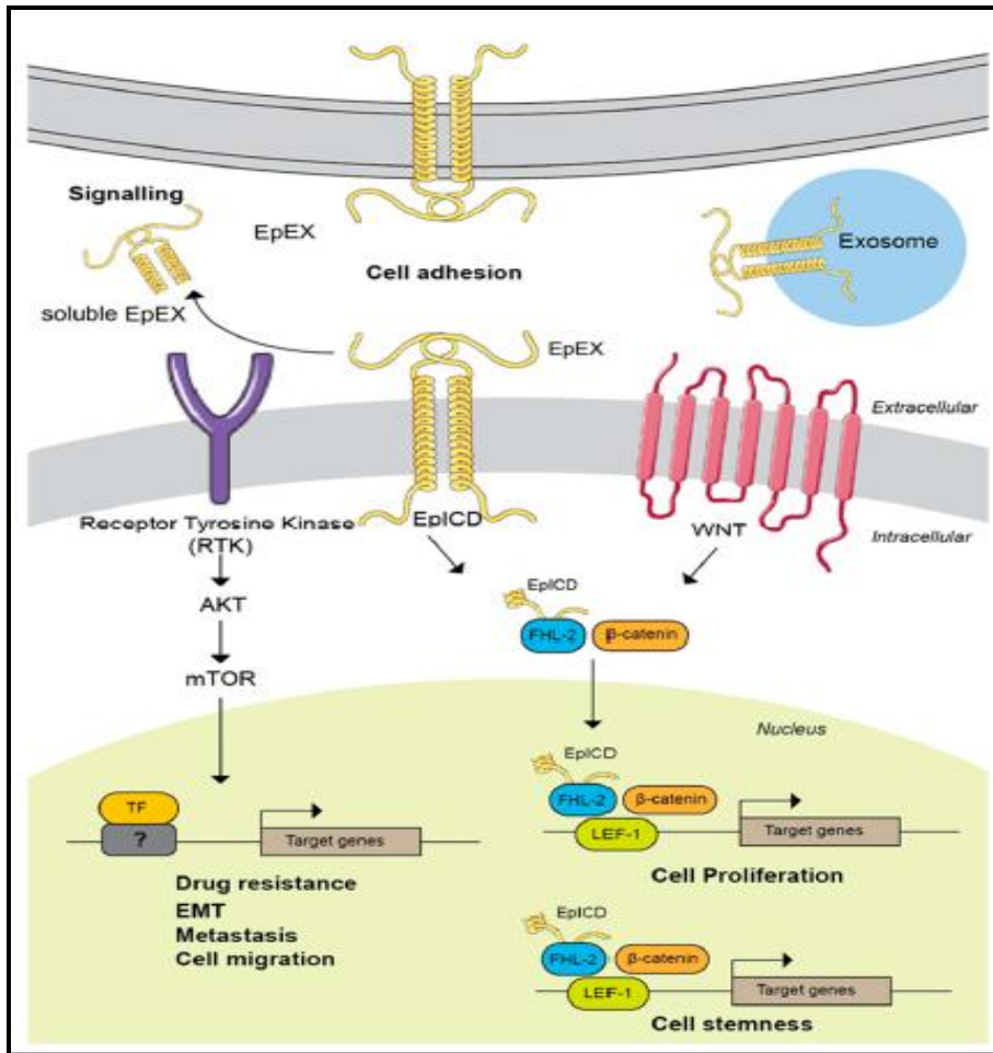
Figure (2): EpCAM localization and modulation of its downstream targets in cancer [8].
