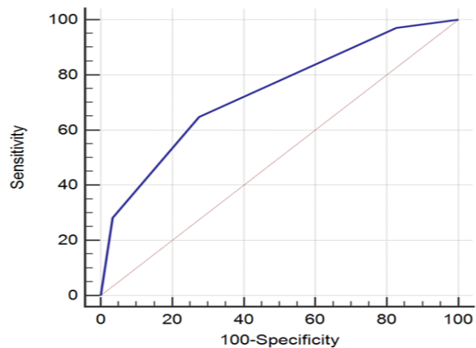
Figure 1: ROC curves for (A) outcomes registry for better informed treatment score and (B) HAS
