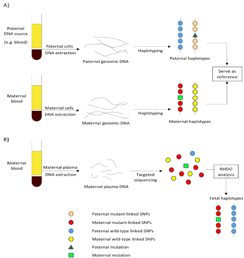
Figure 3: Schematic diagram for the general principle of NIPD of monogenic diseases
