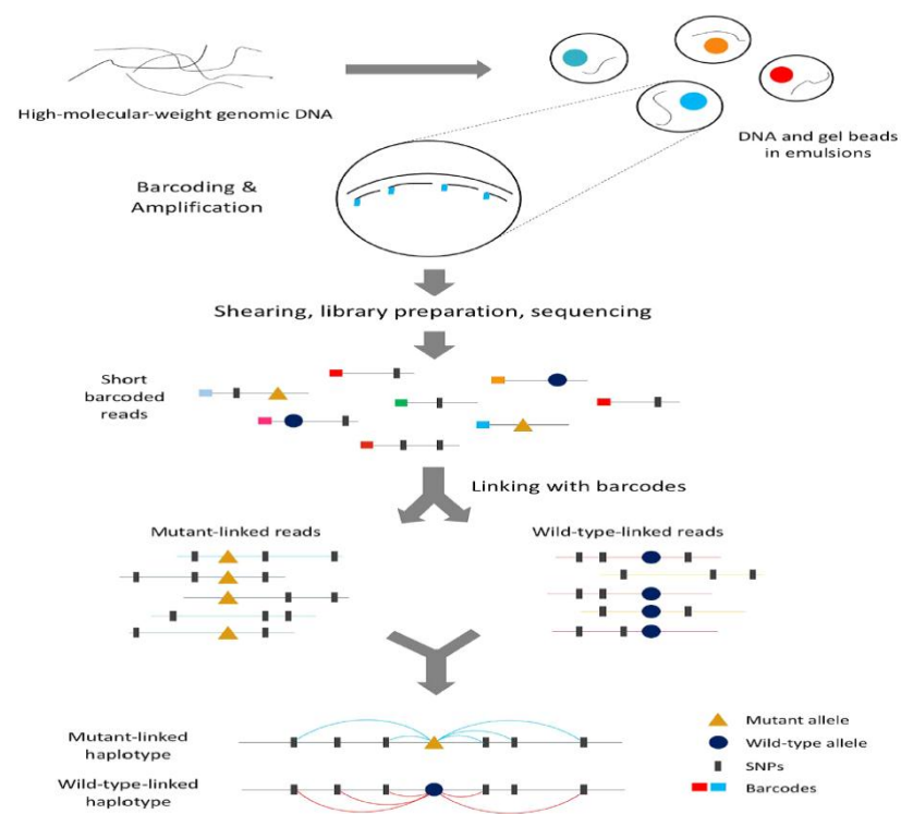
Figure 2: Schematic diagram for the process of linked-read sequencing
