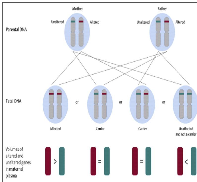
Figure 1: Illustration of relative mutation dosage: red represents the mutated allele and green the
