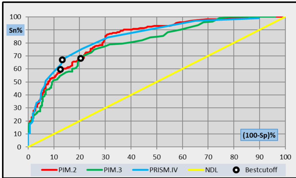
Figure 1. Mortality indices by the area under the receiver operating characteristic curve.
